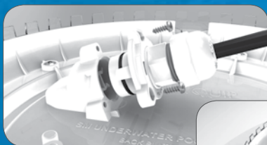
Step 1. Fit the plug kit to the existing cable.
