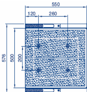
PLANT (Codes 28761, 28760 and 32700)
