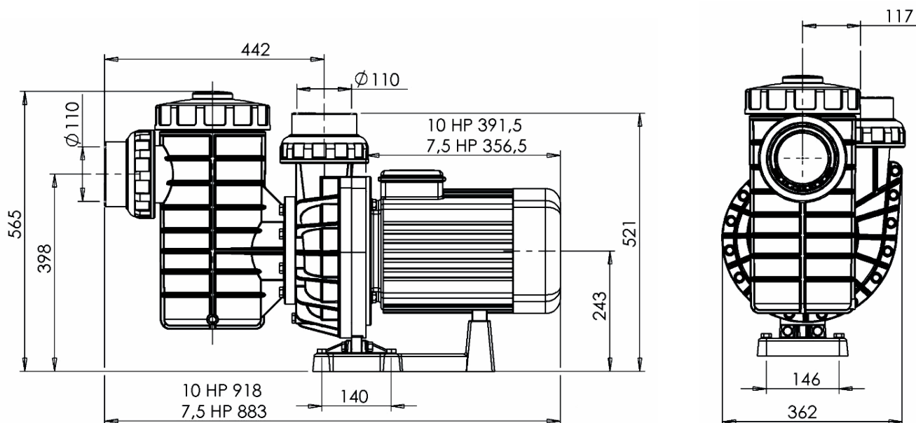
figure 2 - 7,5 – 10 HP Thermoplastic Centrifugal Pumps
