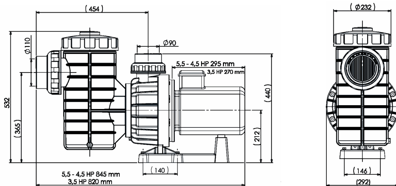
figure 1 - 3, 5 – 4,5 – 5,5 HP Thermoplastic Centrifugal Pumps
