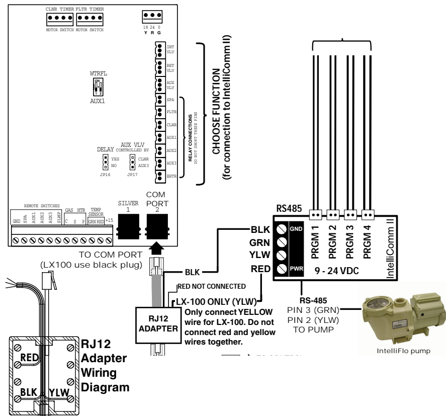
LX100 Motherboard
