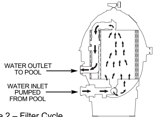
Figure 2 – Filter Cycle
