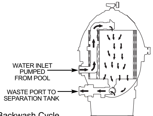
Figure 3 – Backwash Cycle
