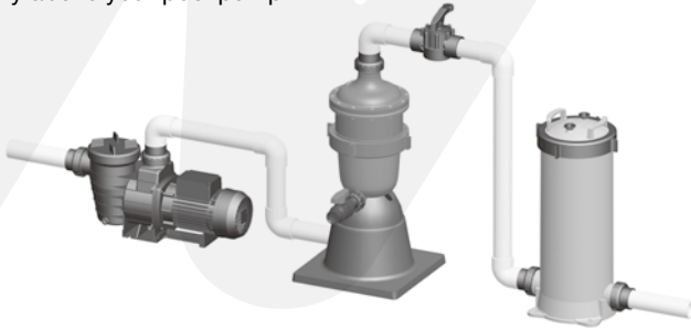
Installation with optional Mounting Stand
