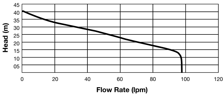
Pool Sweep pump performance chart
